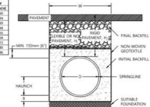
CROSS SECTION VIEW 1:25
