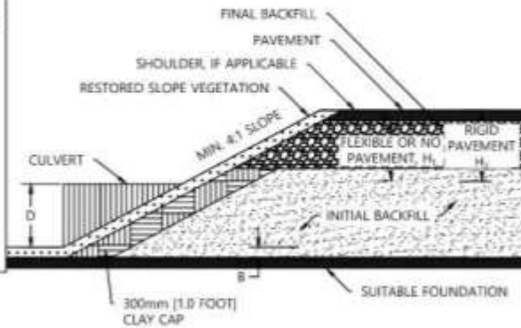
PROFILE VIEW 1:50
