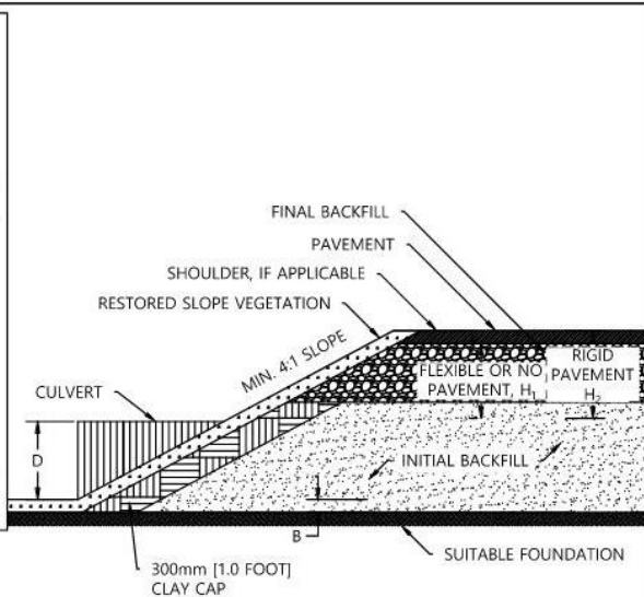
PROFILE VIEW 1:50
