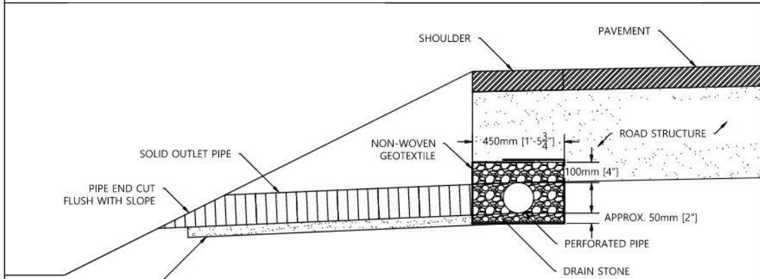
DITCH CROSS SECTION
