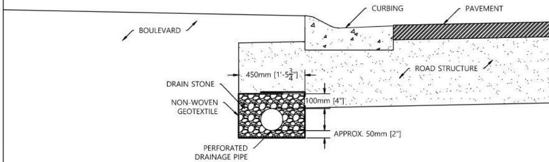
CURB AND GUTTER CROSS SECTION
