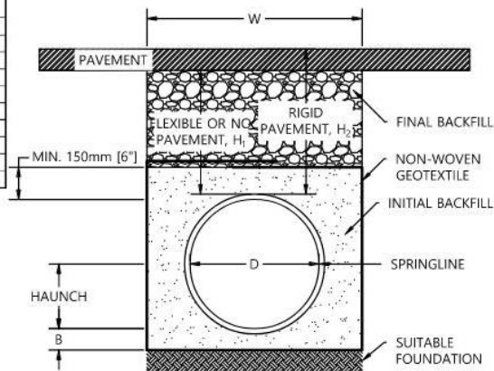
CROSS SECTION VIEW 1:25
